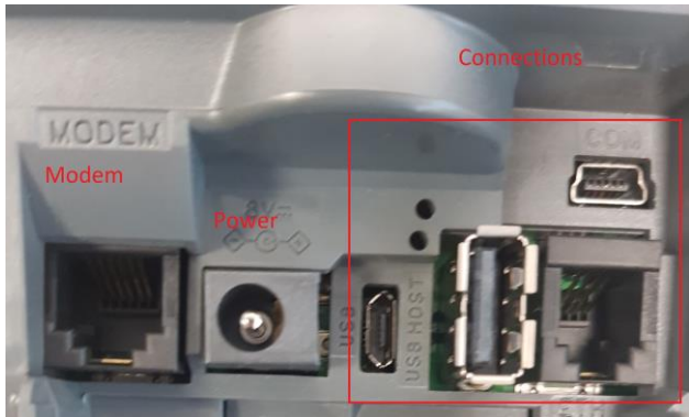
Rear View Casing Open
